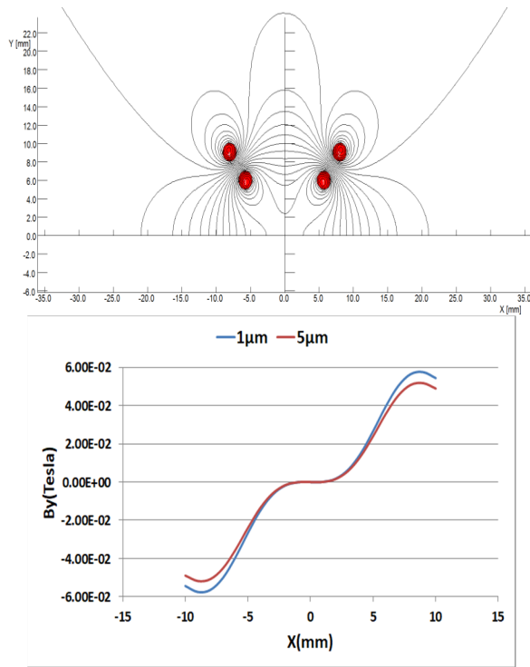
Figure 4: Upper half geometry (Upper) and the resulting field distribution with different coating thicknesses (Lower) of the pulsed nonlinear magnet for the WALS storage ring.
