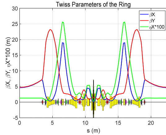
Figure 1: One eighth of the lattice and Twiss parameters for the WALS storage ring.
