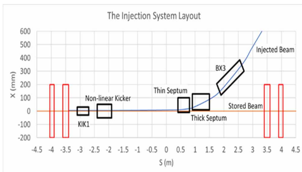
Figure 2: Layout of the injection system for the WALS storage ring.
