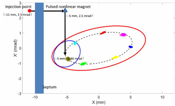
Figure 3: The beam injection procedure (Red ellipse: ring acceptance; blue ellipse: injection beam acceptance; black ellipse: C-S invariant of the injection beam).
