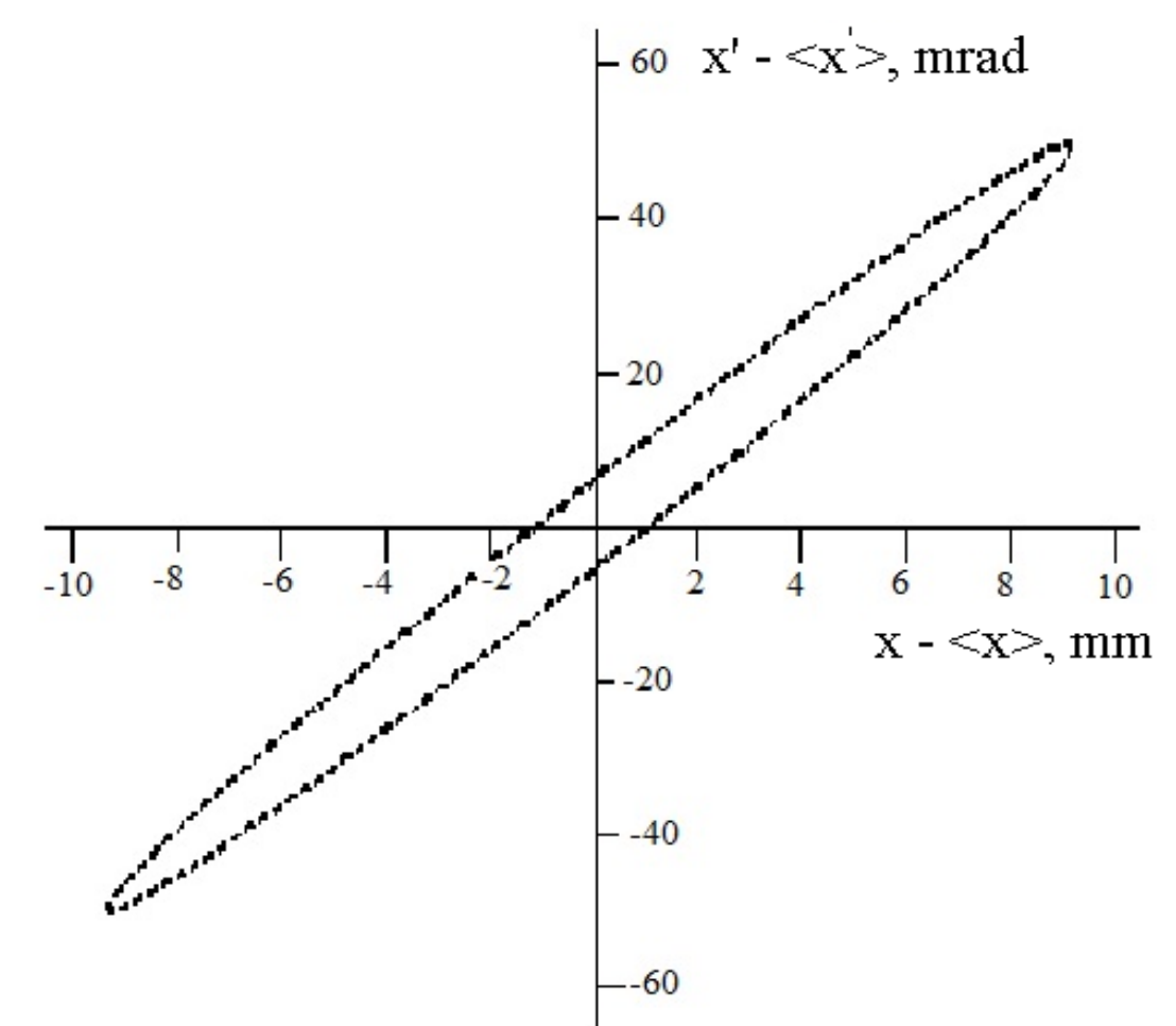
Measured distribution of particles in phase space of a 110 mA total beam (77% proton fraction) at 100 kV.
