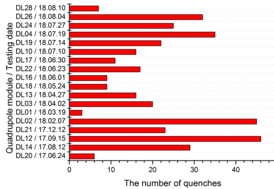
Figure 2: Quenches quantity of the quadrupole doublets.
