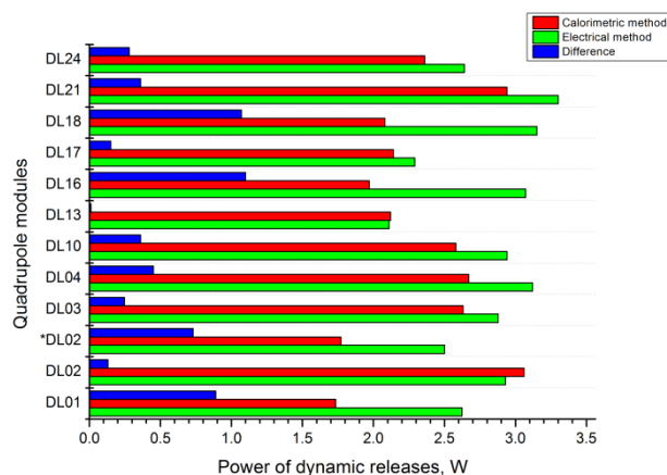
Figure 9: Power of heat releases for the quadrupole doublets.
