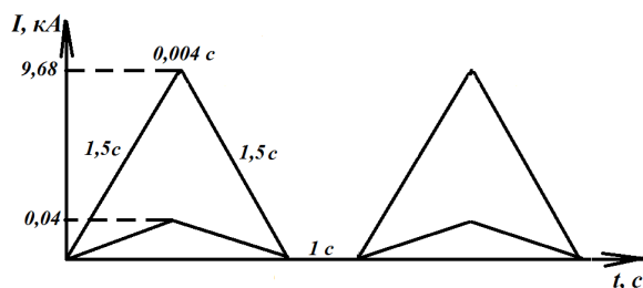
Figure 7: Quadrupole magnet's current cycle.
