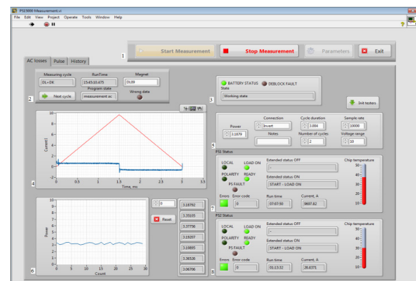
Figure 6: The program for automation of dynamic heat releases measurement: 1 - Controlling buttons, 2 - Measurement status bar, 3 - Status of energy evacuation switch, 4 - Data graph, 5 - Cycle parameters, 6 - Heat releases power graph, 7 - Status of first power supply, 8 - Status of second power supply.
