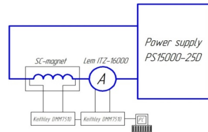
Figure 5: The scheme of dynamic heat releases measurement.
