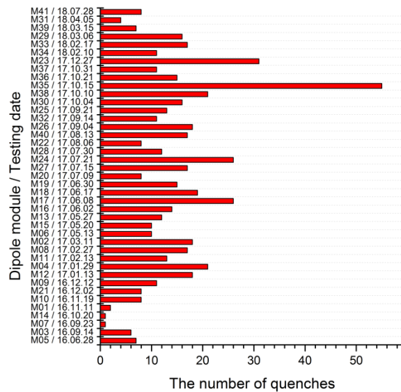
Figure 3: Quenches quantity of the dipole magnets.
