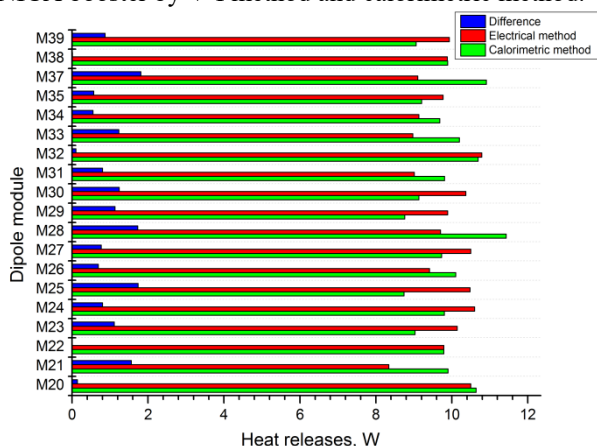
Figure 8: Power of heat releases for the dipole magnets.
