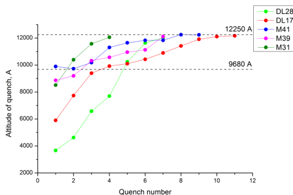
Figure 4: The current altitudes of quenches at SC magnets DL28, DL17, M41, M39, M31.
