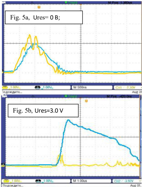
Figure 5: Trigger current, measured by RC1 (yellow trace) and RC2 (blue trace). Thyatron TDI3-100k/45H. Anode voltage U_a = 0 kV, R_{ad} = 48 Ohm.
