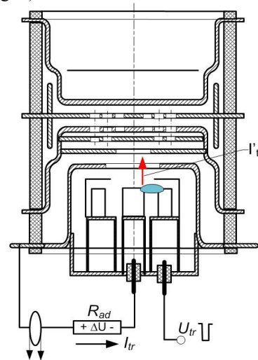
Figure 4: Circuit schematic of thyatron TGI3 - 10k/50 with thermionic cathode with cathode modules placed along the circumference and in the center.
