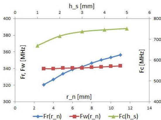
Figure 5: Calculated working F_w , spurious F_r and F_c modes as a functions holder's length.
