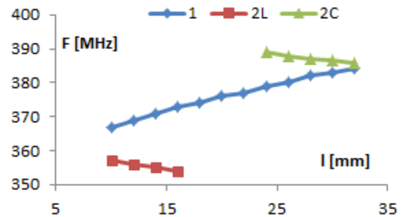
Figure 7: Experimental data for spurious modes as a functions of reactance of holder.
