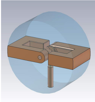
Figure 4: Model of an intermediate electrode holder in accelerating structure.
