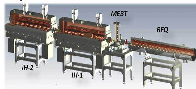
Figure 2: HILAC scheme.
