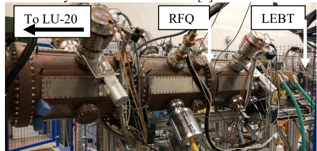
Figure 4: The new RFQ fore-injector.
