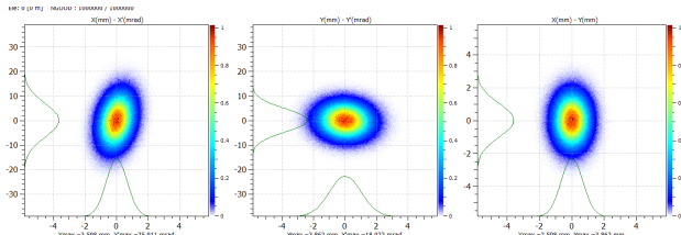
Figure 4: Input phase-space ellipses of the transport channel.
