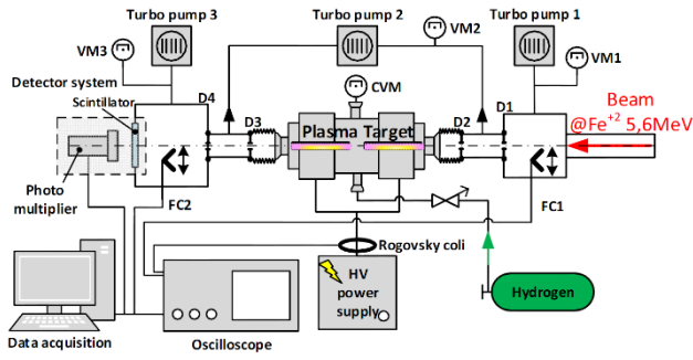
Figure 3: Vacuum system and diagnostic equipment, D1-4 – diaphragms of differential pumping system \varnothing = 1\text{-}3\text{mm} , VM1-3 – vacuum meters, CVM – gas independent vacuum-meter, FC1-2 – Faraday cups.
