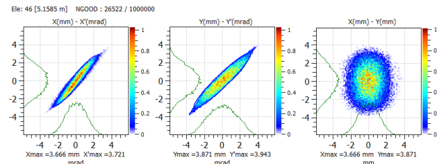
Figure 7: Output phase-space ellipses of PT.
