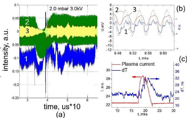
Figure 8: (a,b) 1 - raw photomultiplier signal, 2 - accelerator RF signal, 3 - Fourier correction of row signal. (c) - plasma current (left) and microbunch shift dT (right) compared in time.
