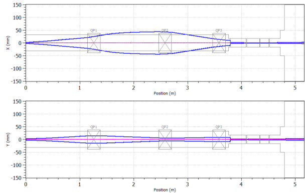
Figure 6: Multiparticle envelopes in x and y directions.
