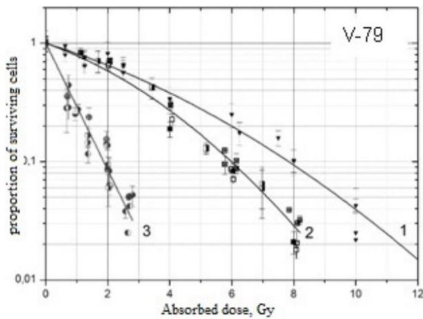
Figure 1: The curves of the survival of the chinese hamster cells of the V-79 line under the action of the ^{12}\text{C} ion beam in the plateau region (curve 2), unmodified Bragg peak (curve 3) and ^{60}\text{Co} \gamma -radiation (curve 1).
