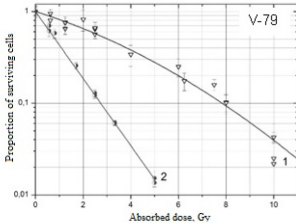
Figure 2: The survival curves of the chinese hamster cells of the V-79 line under the action of neutron radiation in the absence of proton balance (curve 2) and gamma radiation of ^{60}\text{Co} (curve 1).
