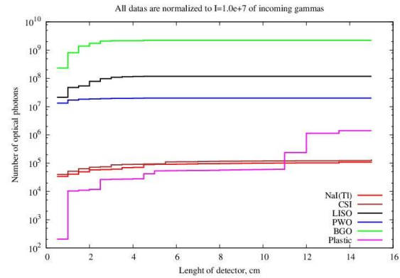
Figure 5: The light output of the detecting element of the matrix, made of different types of scintillator.
