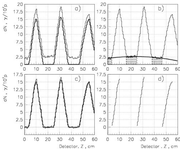
Figure 4: The distribution along the longitudinal coordinate of prompt \gamma -rays intensity at the detector. Idealized distribution (thick line) - without taking into account the contribution of neutrons using absolutely black collimators; realistic distribution (thin line) - taking into account the neutron background and realistic WNiFe-collimators): a) - realistic and idealized distribution; b) definition of the
