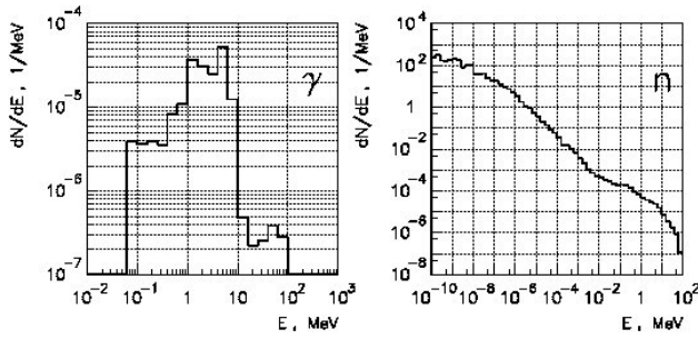
Figure 3: Energy distributions of prompt \gamma -rays and neutrons from a primary proton beam with an energy of 100 MeV.
