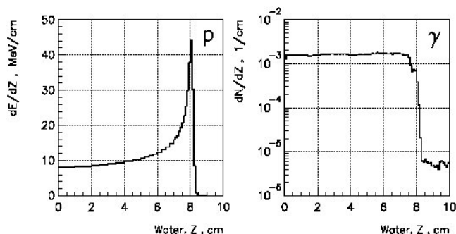
Figure 1: The deep distribution of energy deposition and the density of prompt \gamma -rays production from the primary proton beam with an energy of 100 MeV in the water phantom.
