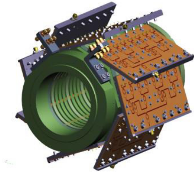
Figure 4: Pickup/kicker structure by FZ Julich.
