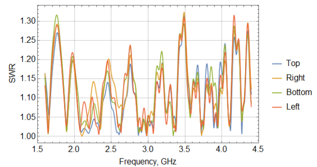
Figure 13: Plot of kicker SWR.
