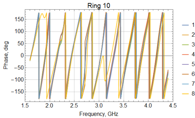
Figure 9: Plot of phase for rings.
