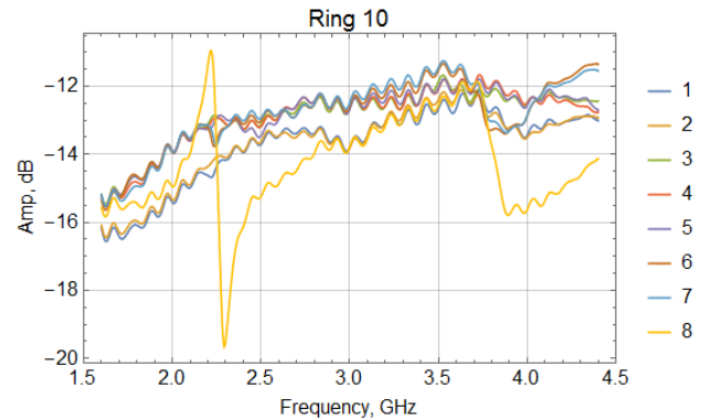
Figure 8: Plot of amplitude for rings.
