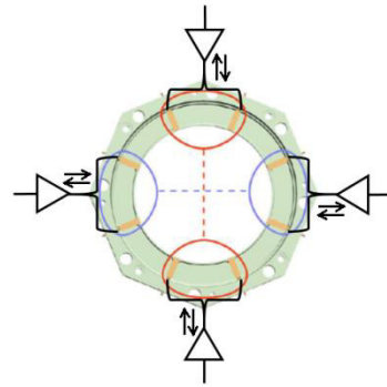
Figure 12: Kicker power feed scheme.
