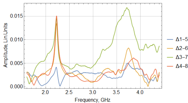
Figure 10: Amplitude of the difference signal from the corresponding azimuths.
