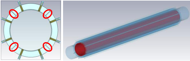
Figure 5: Cut structure with ceramic vacuum chamber inside rings.
