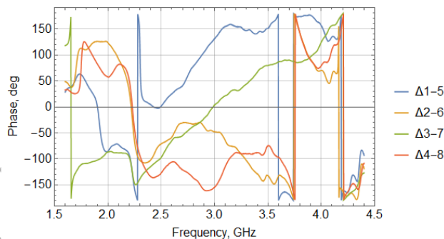
Figure 11: Phase of the difference signal from the corresponding azimuths.
