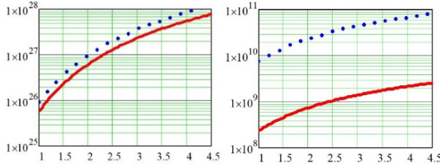
Figure 2: a) Collider Luminosity vs ion energy in Au x proton mode. Solid line: L(E_i) calculated by Formula (7), and the dotted line – by Formula (1). b) Particle number per bunch vs E_i . Solid line – N_i(E_i) , dotted line – N_p(E_i) .
