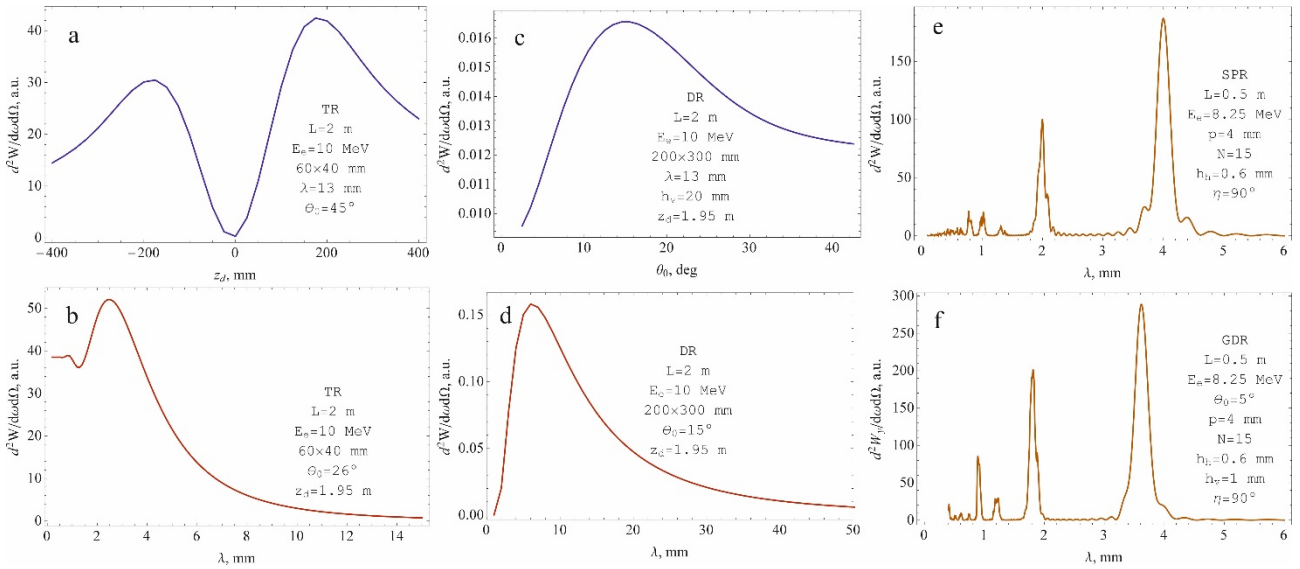
Figure 3: The simulation result examples of different radiation types: TR angular distribution (a), DR orientation distribution from one plate (c), TR spectrum (b), DR spectrum from one plate (d), Smith-Purcell radiation (e) and grating diffraction radiation (f) spectra ( h_H and h_V are the impact parameters, N is the number of periods, p is the grating period).
