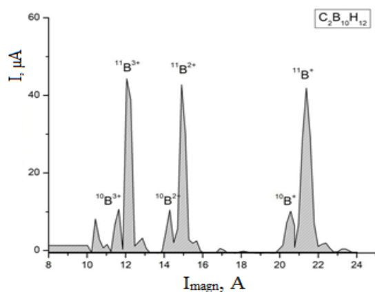
Figure 3: Charge state distribution of the extracted B ions.
