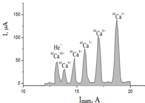
Figure 8: Charge state distribution of the extracted Ca ions (SC).
