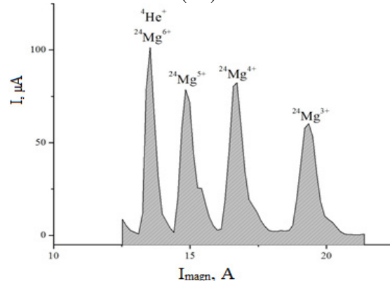
Figure 7: Charge state distribution of the extracted Mg ions (EC).
