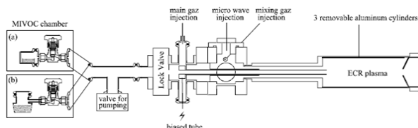
Figure 1: Schematic view of MIVOC chamber connection to ECR ion source.
