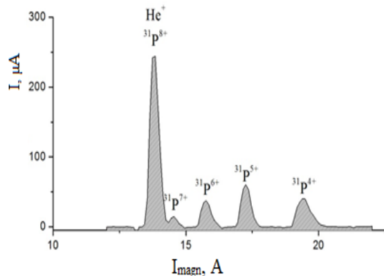
Figure 9: Charge state distribution of the extracted P ions (SC).
