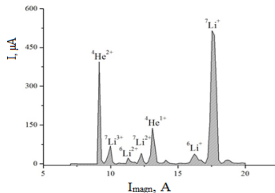
Figure 6: Charge state distribution of the extracted Li ions with the standard crucible (SC).
