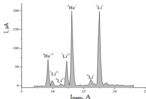
Figure 5: Charge state distribution of the extracted Li ions with the enlarged crucible (EC).
