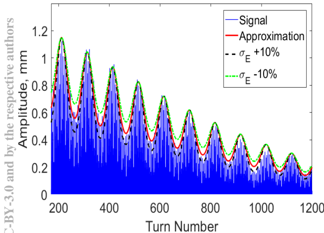
Figure 2: Envelope of coherent oscillations.
