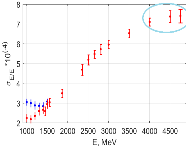
Figure 4: Measured energy spread.
