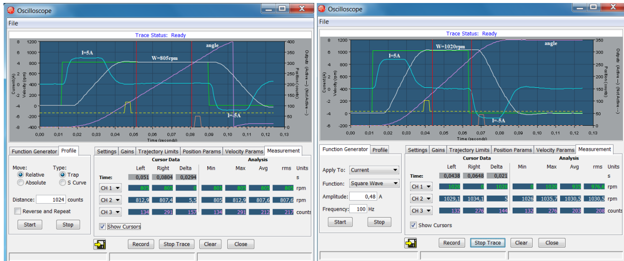
Figure 4: Oscillograms of acceleration, uniform motion and braking of the carbon fiber for a horizontal and vertical wire scanner.
