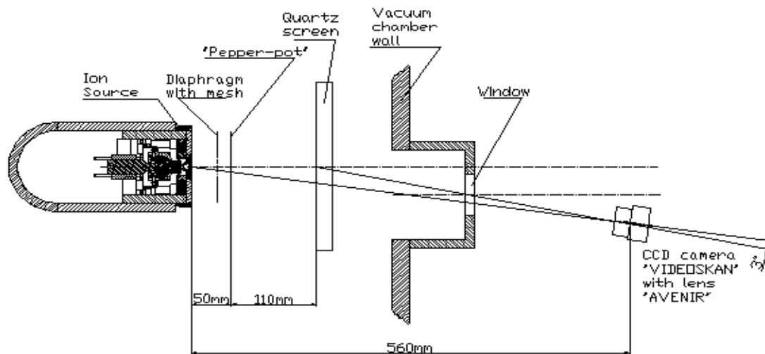
Figure 1: Scheme of the emittance measuring device.
