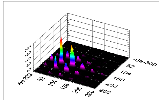
Figure 2: The signals distribution from the pixels of the matrix after the background subtraction.
