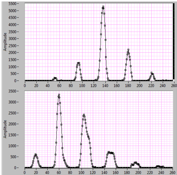
Figure 3: Intensity distribution after integration of the distribution function f(x,y) along X or Y axis.
