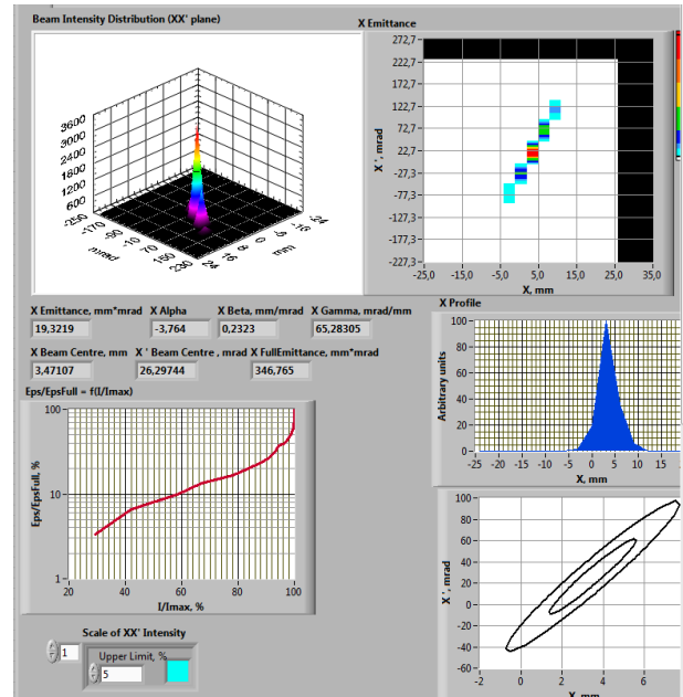
Figure 4: Results of the data processing in XX' plane.
