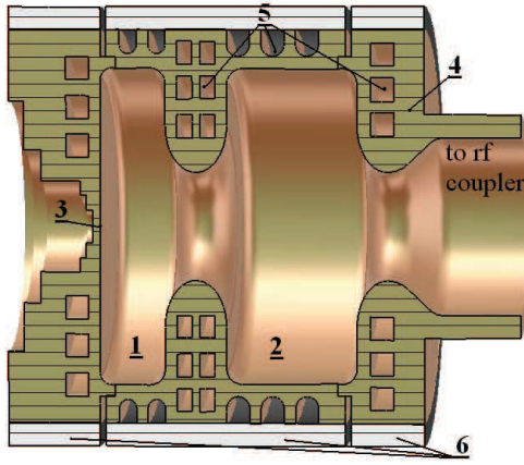
Figure 2: Simplified model of the gun cavity. 1 - half cathode cell, 2 - full cell, 3 - position of photo cathode, 4 - cavity copper body, 5 - cooling channels, 6 - stainless steel jacket.
