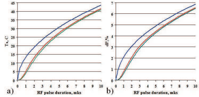
Figure 3: Time dependence of maximal temperature rise of the surface T_{smax} (a) and relative increase of RF losses (b) for rectangular (blue traces) and accretive with \tau_{c1} (red traces) or \tau_{c2} (green traces) P_l pulse.
