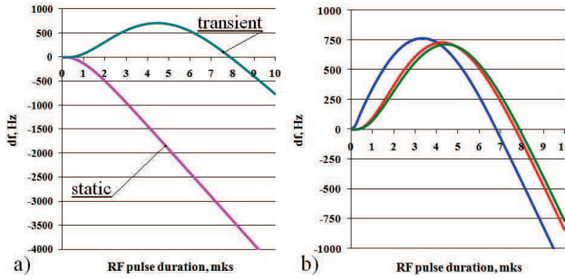
Figure 5: Cavity detuning during accretive ( \tau_{c1} ) P_l pulse for static and transient approximations (a) and transient detuning for rectangular (blue curve), accretive with \tau_{c1} (red curve) or \tau_{c2} (green curve) P_l pulses (b).
