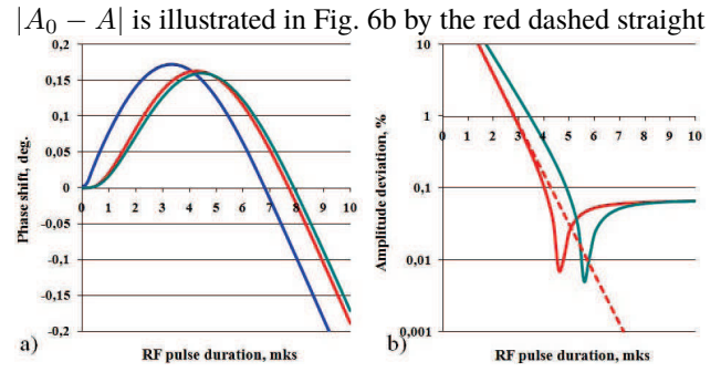
Figure 6: Temporal dependence of the phase shift of RF oscillations for rectangular (blue curve), accretive with \tau_{c1} (red curve) or \tau_{c2} (green curve) P_l pulses (a) and absolute value of amplitude deviations for accretive with \tau_{c1} (red curve) or \tau_{c2} (green curve) P_l pulses (b).
