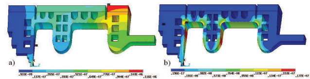
Figure 4: Distribution of displacements after \tau = 4.5 \mu s accretive ( \tau_{c1} ) RF pulse for static (a) and transient (b) approximations.
