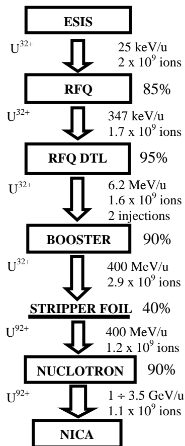
Fig. 1. Injection chain of the NICA collider based on ESIS source and RFQ linac.
