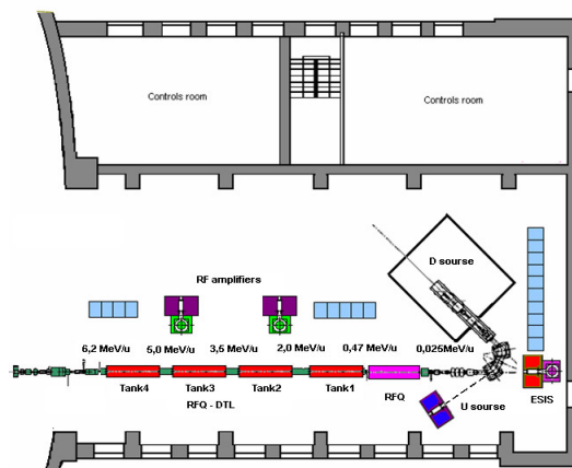
Fig. 2. Injector location in the existing building.
