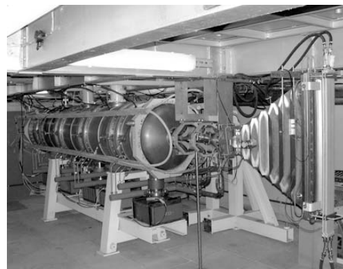
Figure 4: Accelerating structure with beam scanning system.
