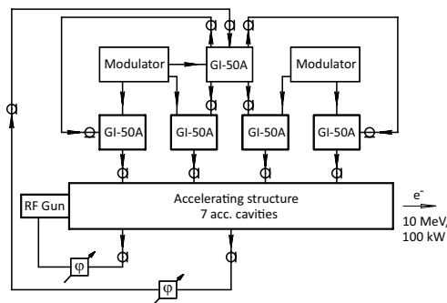
Figure 1: ILU-14 accelerator block diagram.
