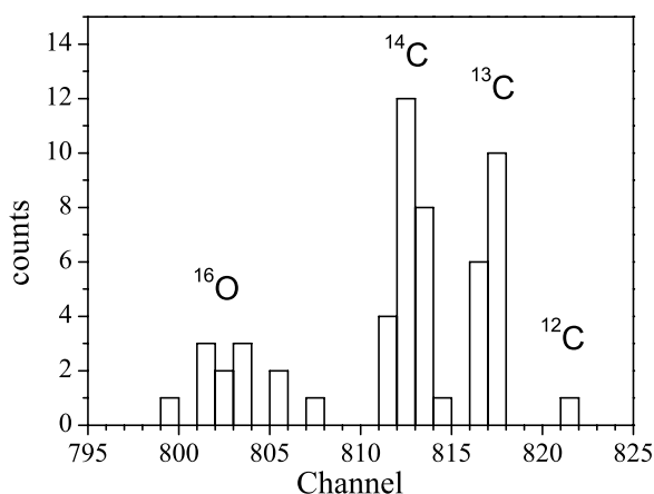
Figure 3: TOF ion counts with fixed HE magnet setting for 14 C passing.
