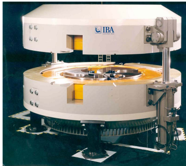
Fig. 3 C235 IBA cyclotron for proton therapy.
