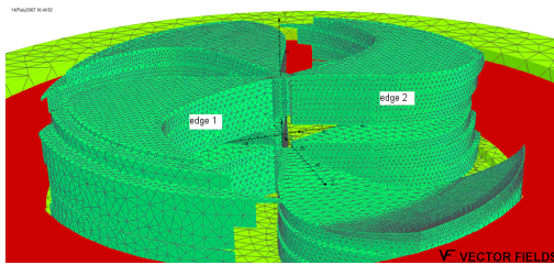
Fig.8 Simulation of the magnetic field.
