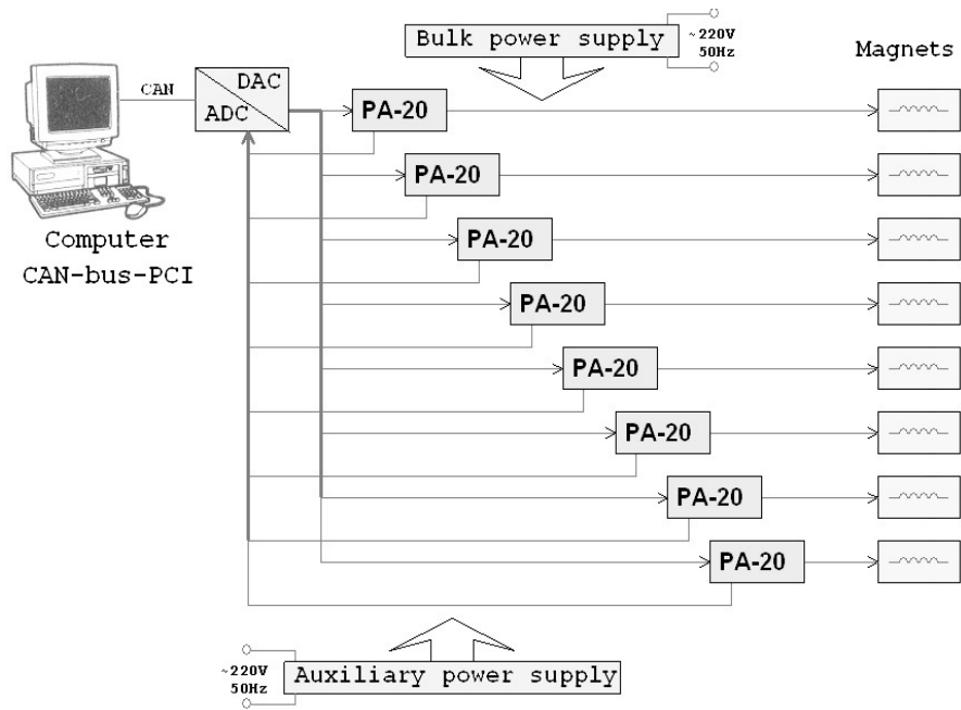
Figure 2: Multichannel system of Power Amplifiers for Magnets.
