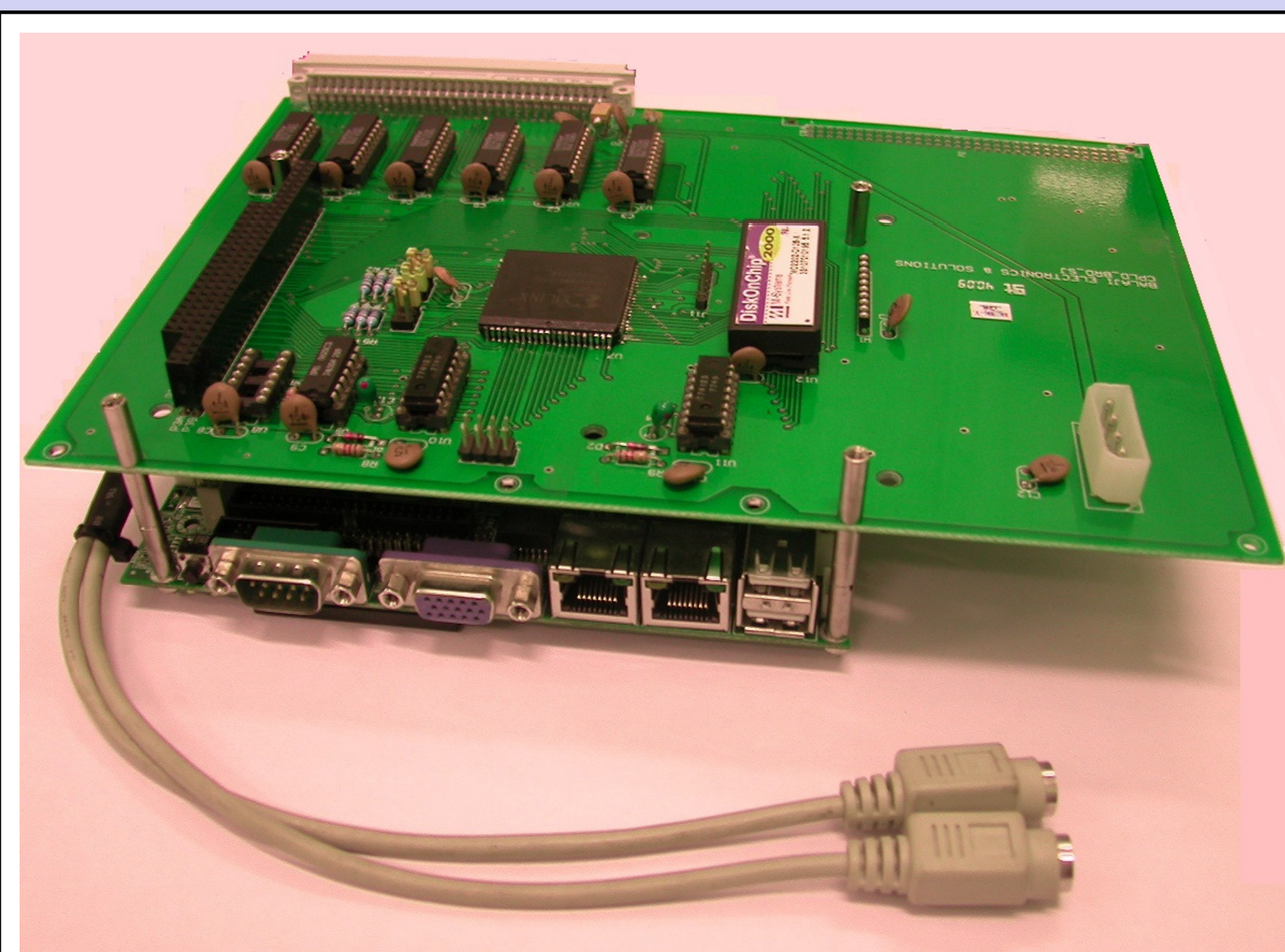
Figure 2: System Controller Module.
