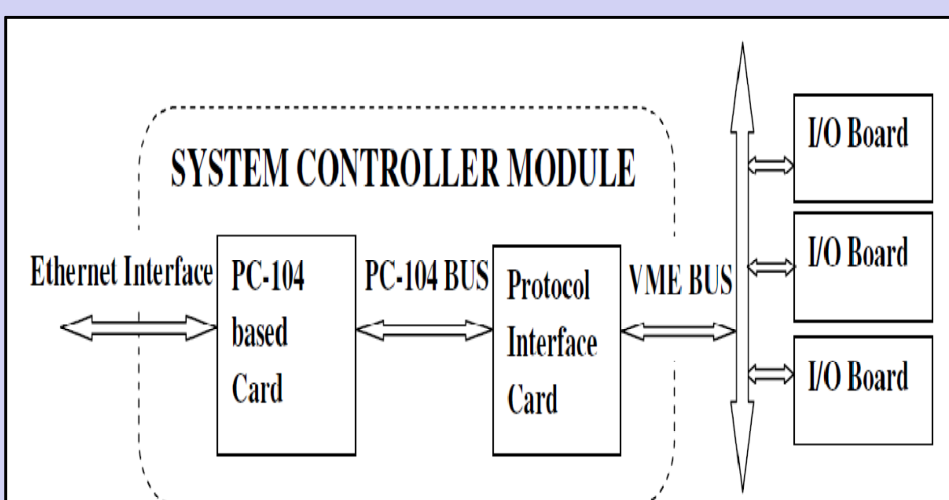
Figure 1: System Controller Module Block Diagram.
