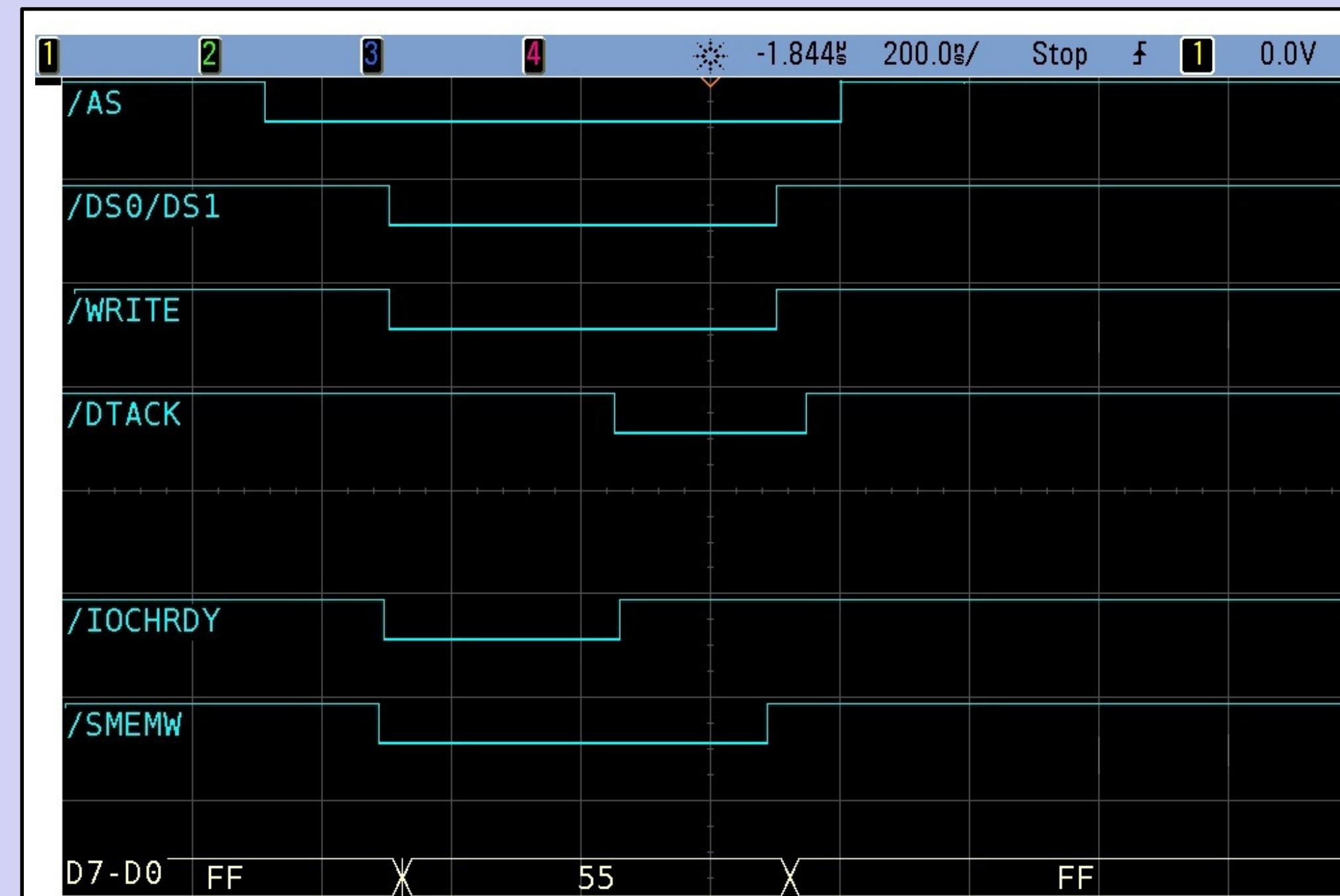
Figure 3: Timing diagram of VME and PC-104 Signals
