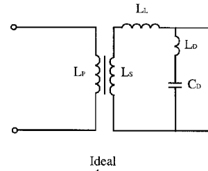
Figure 1. Equivalent circuit for the pulse transformer.
