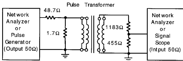
Figure 3. Test circuit.
