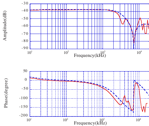
Figure 4. Amplitude and phase for the pulse transformer as a function of frequency.
