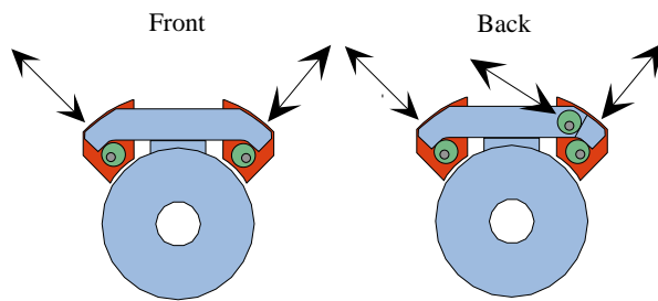
Figure 3: Cam arrangements at the front and back of the cryostat.
