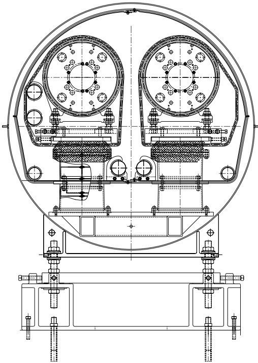
Figure 2: The cryostat cross section of the High Beta Magnets. The insulating posts and the stands are shown.
