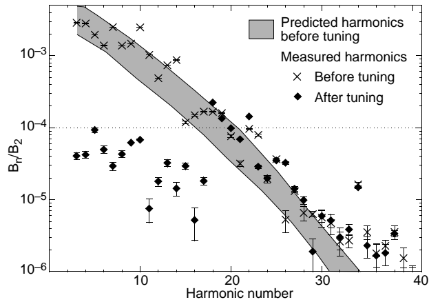
Figure 2. The harmonic content of the prototype magnet before and after the quadrupole blocks are radially adjusted. The quadrupole and dipole harmonics are off-scale and hence not shown. The inner radius of the magnetic material is 7.4 cm. These harmonics are shown at a radius of 5.9 cm. The gray area is the region for the harmonics predicted by the computer model before tuning.
