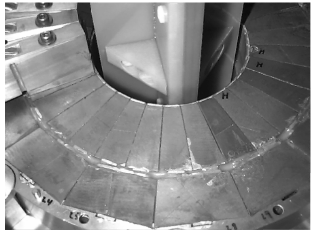
Figure 3. The prototype slice with the harmonic measuring coil in place. The Al tabs have been machined off. Some of the quadrupole block support arms are shown on the left side of the picture.
