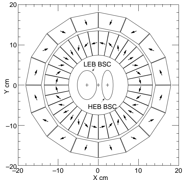
Figure 1. Block dimensions and magnetization angles of the blocks that make the field in the Q1 magnet. The BSC ellipses are at the end farthest away from the IP ( z=2.1 m).
