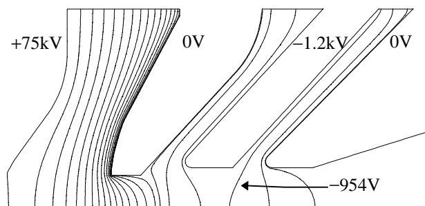
Figure 4. Equipotentials from the POISSON solution of the ion-source accelerating column. The equipotential spacing is dense near 0 Volts and sparse near 75 kV.
