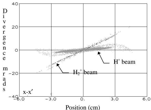
Figure 1. Simulated distribution of H^+ and H_2^+ at the position of the EMU. The solenoid lenses do not focus the H_2^+ beam as strongly as the H^+ beam, so the H_2^+ beam diverges more than the H^+ beam. This beam contains 118 mA of H^+ and 12 mA of H_2^+ . The rms emittance of the simulated H^+ beam is 0.028 cm-mrad. (If viewing in color, H^+ ions are green and H_2^+ ions are red.)
