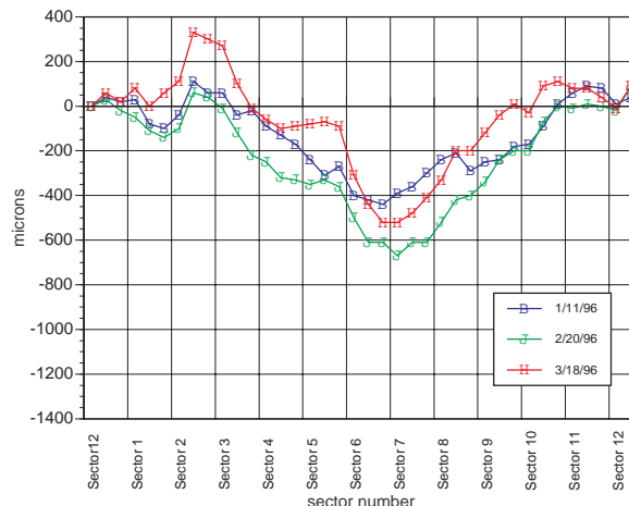
Figure 2a: Elevation changes around the storage ring
