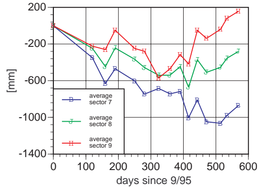
Figure 3c: Elevation changes at the storage ring
