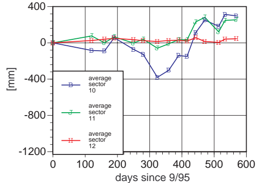
Figure 3d: Elevation changes at the storage ring
