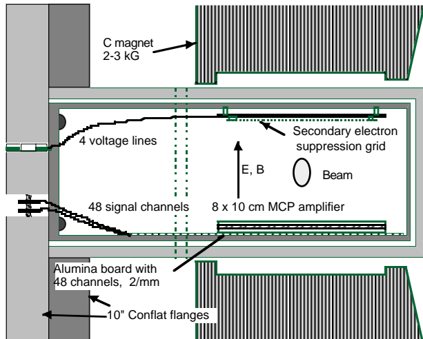
Figure 1. Cross section of IPM. View is looking down the beamline. In this experiment the orientation was rotated 90° CW so the detector mounting flange was horizontal.
