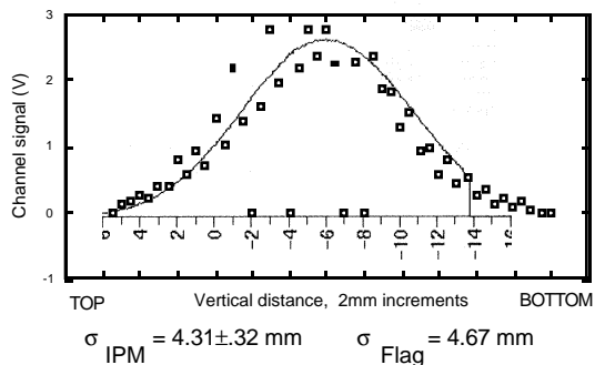
Figure 3. A Gaussian fit to the fluorescent screen profile, solid curve, overlaid the data collected from the IPM. The screen was located 2m downstream and the beam was diverging.
