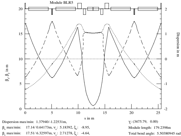
Figure 3: The Flexible Momentum Compaction Module of the 50 GeV demonstration storage ring
