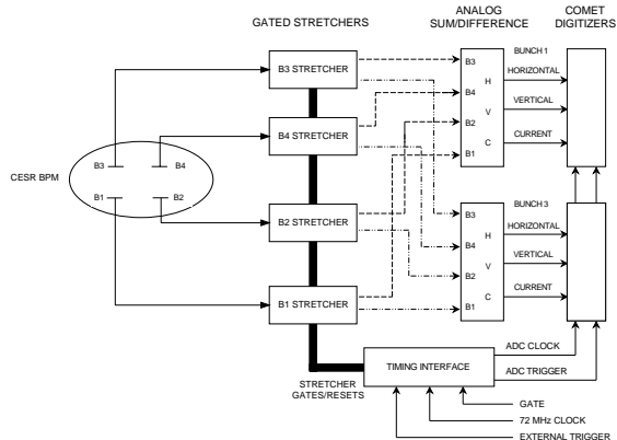
Figure 1: The turn-by-turn data acquisition system. Four beam position monitor signals are gated, stretched, and combined to provide bunch-by-bunch horizontal, vertical, and current signals. The system shown provides signals for one beam species. Another identical system provides signals for the other species.
