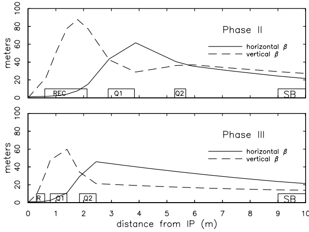
Figure 2: Upper plot shows optical functions in Phase II IR. With superconducting quadrupoles (Q1 and Q2) in Phase III, \beta_v^* \sim 10\text{mm} and \beta_v at the parasitic crossing 7ns(2.1m) from the IP is 30m.
