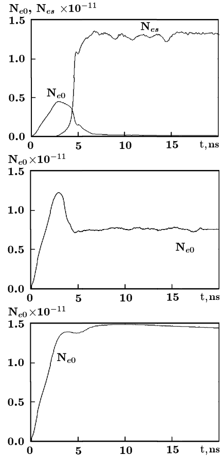
Figure 2: Dynamics of store of electrons inside the gap for the above mentioned cases.
