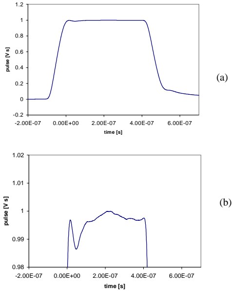
Figure 3: Measured pulse of a modified kicker magnet (a). The lower graph shows the field ripple in more detail (b).
