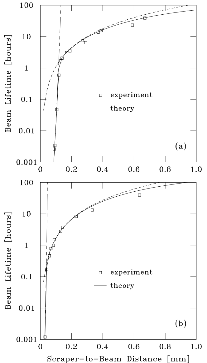
Figure 1: Vertical scraper results at low current: 21mA at 2.584 GeV. Two components of the theory curve are also illustrated, the quantum lifetime (section line) and the nuclear Coulomb scattering lifetime for the vertical (dashed line). (a) \sigma_y=20 \mu\text{m} ; (b) \sigma_y=7 \mu\text{m} .
