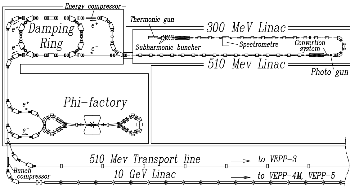
Figure 4. Layout of Injecor complex
