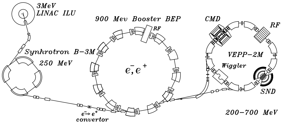
Figure 1. Layout of VEPP-2M complex
