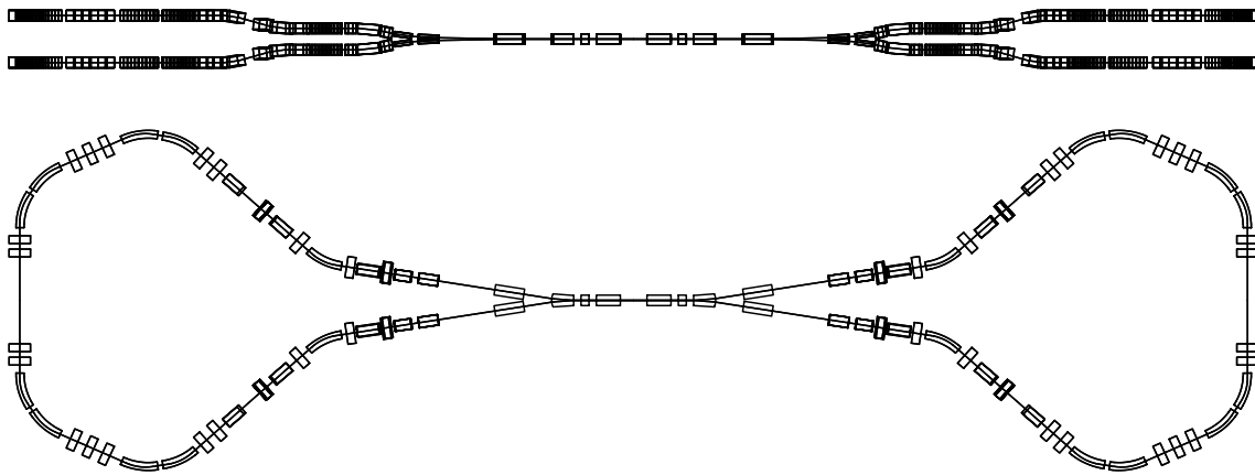
Figure 5. Layout of Phi-factory
