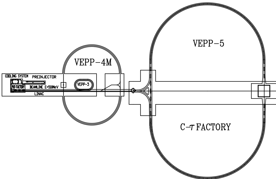
Figure 3. Layout of VEPP-5 complex
