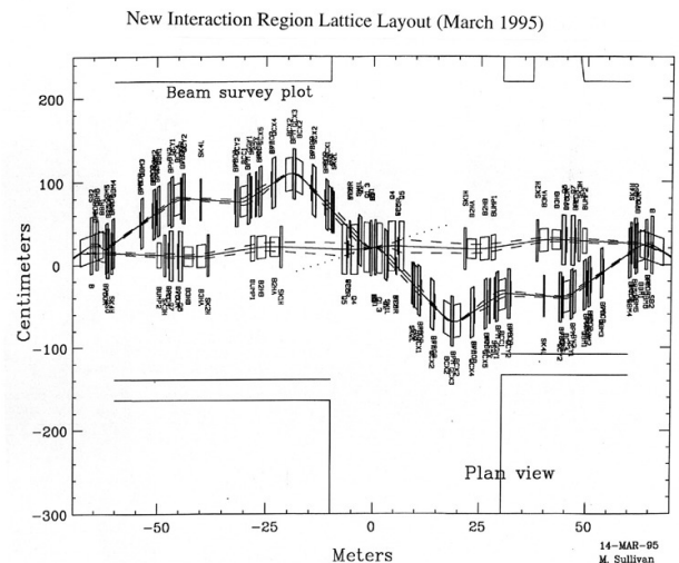
Figure 6 Interaction region lattice layout.
