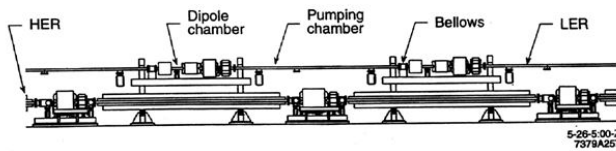
Figure 2 Cell layout
