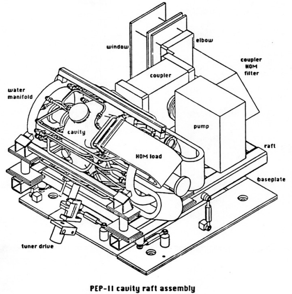
Figure 9 PEP II cavity raft assembly.
