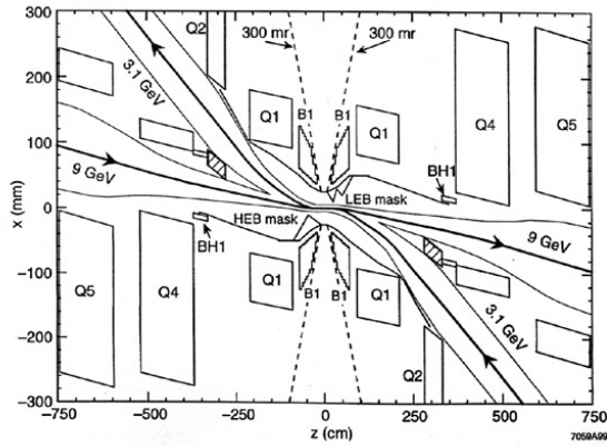
Figure 7 Beam separation at the interaction point.
