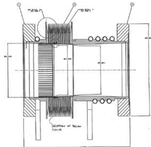
Figure 4 HER Vacuum chambers: a) dipole , b) quadrupole, c) arc bellows, and d) straight section bellows.
