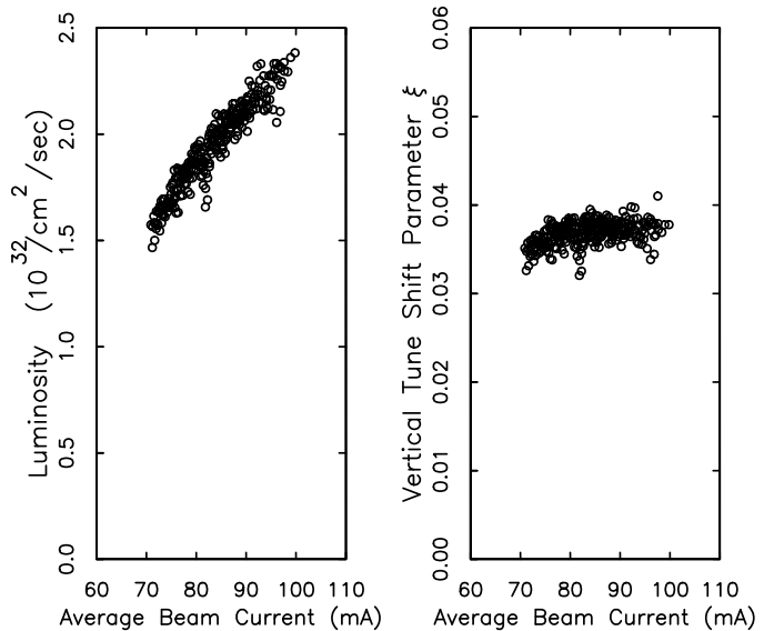
Figure 4. Luminosity versus beam current with nine bunches per beam and crossing angle of \pm 2.1 \text{mrad} .
