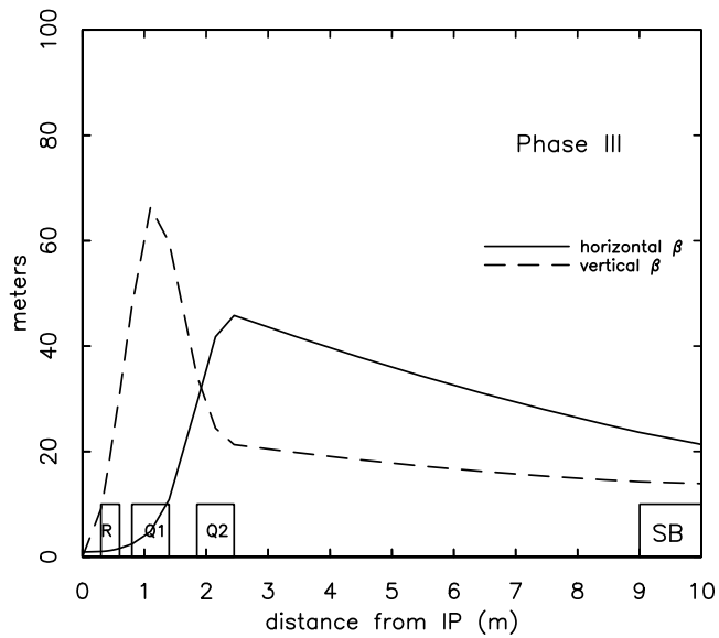
Figure 7. Optical functions in the superconducting IR.
