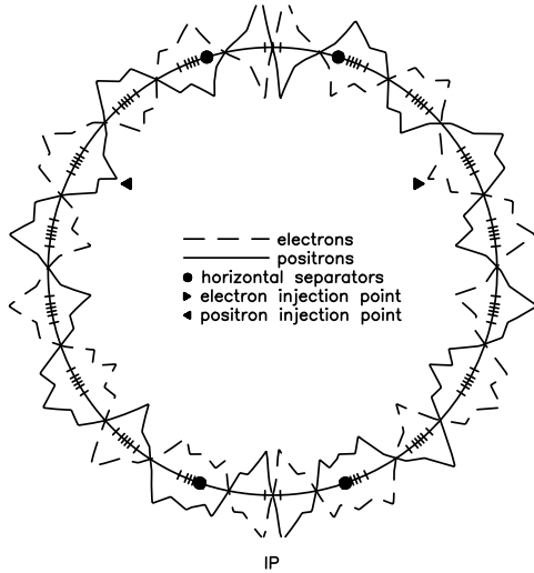
Figure 2. Electron and positron closed orbits in crossing angle operation. The crossing angle is \pm 2.3 mrad . Tic marks along the circumference indicate parasitic crossings with 9 trains with the 2 bunches/train spaced 28ns apart.
