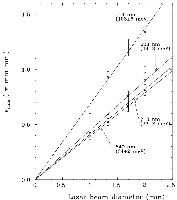
Figure 2. The rms-emittance as a function of laser beam diameter for several laser wavelengths. The inferred thermal energies are shown in parenthesis.
