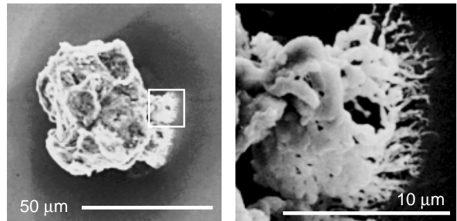
Figures 3a & 3b: A thermal defect (copper)
