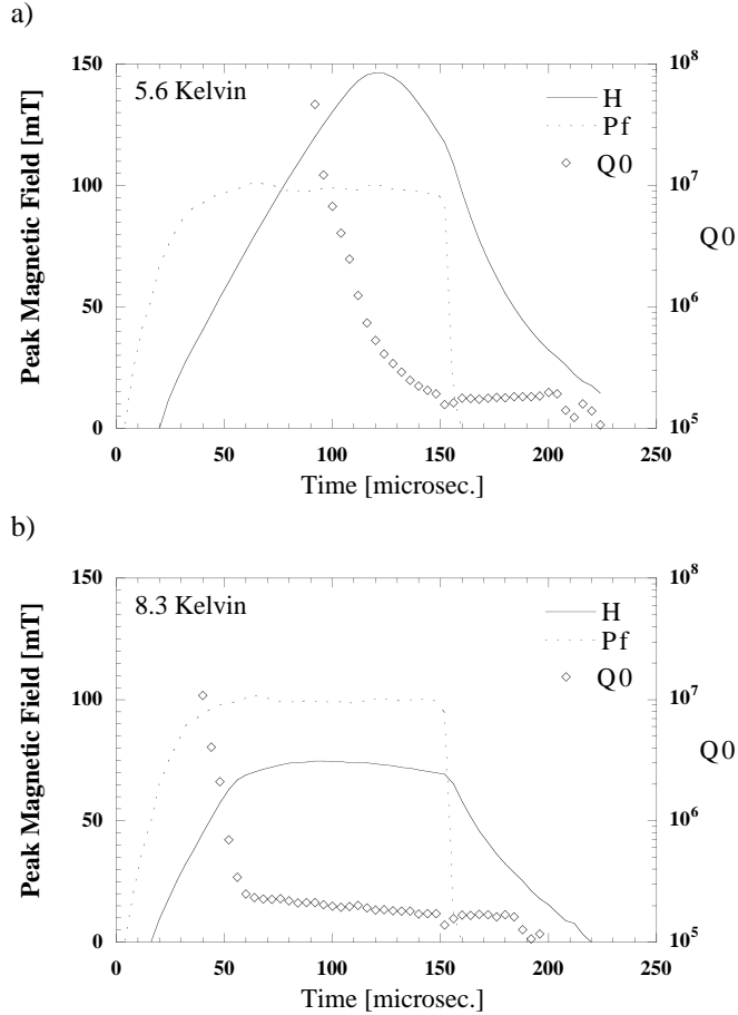
Figure 1. Pulses to the cavity causing thermal breakdown at a) 5.6 K and b) 8.3 K. Peak forward power was 340 kW for both pulses. Forward power is shown with arbitrary units.
