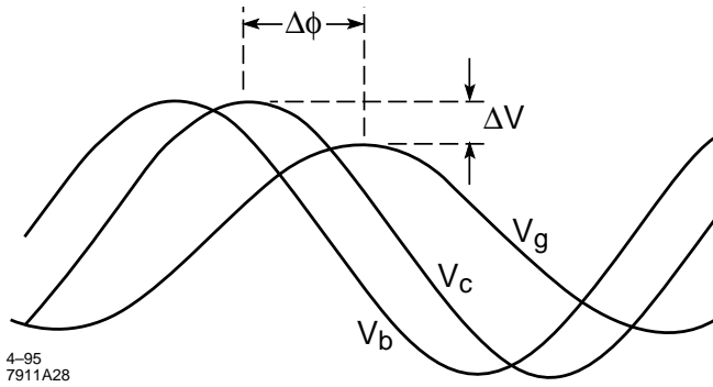
4-95 7911A28 Figure 3. Cavity voltages highlighting errors in the voltage \Delta V and phase \Delta\phi resulting from beam extraction.
