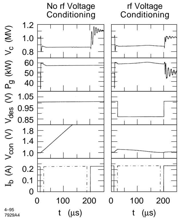
4-95 7929A4 Figure 4. Cavity regulation and voltage transient reduction in the SLC with and without rf conditioning in the event of a missing pulse. Plotted as a function of time are the cavity voltage V_c , the klystron output power P_g , the reference input to the amplitude feedback loop V_{des} , the amplitude feedback control voltage V_{con} , and the rf current I_b . The dot-dashed curve in I_b indicates the missing pulse.
