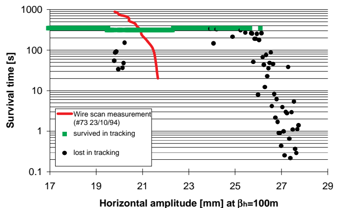
Figure 5. Dynamic aperture at WP2, natural ripple only.
