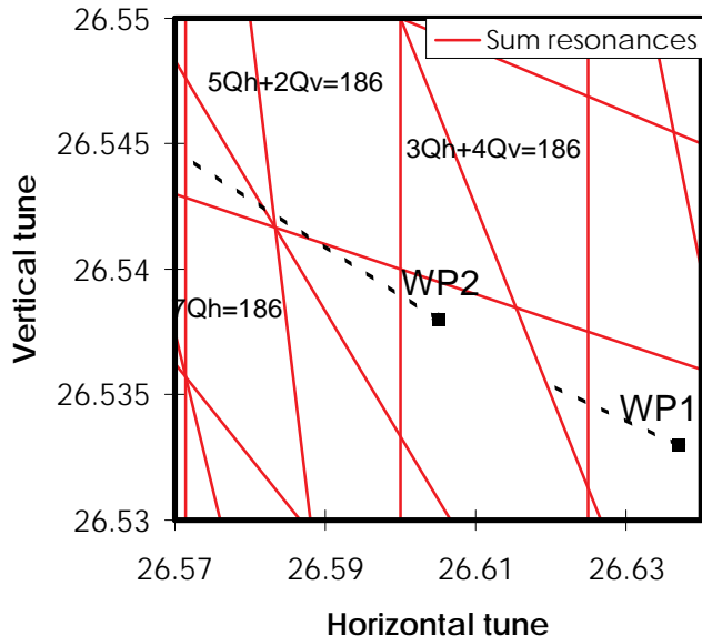
Figure. 1. Tune diagram with sum resonances up to order 11 and both working points before and after the kick. The detuning is directed towards smaller horizontal and larger vertical tune values. At the last tune values large scale losses take place.
