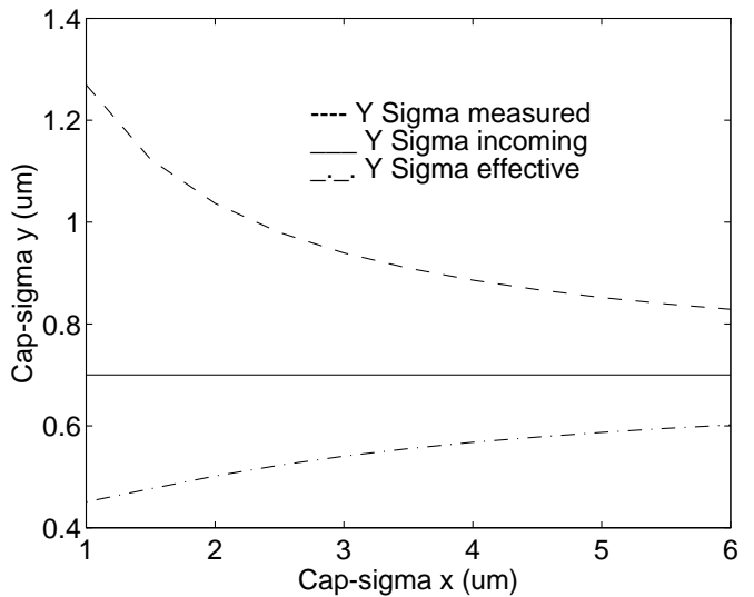
Fig. 5: \Sigma_y , (measured) and \Sigma_y , (effective) versus \Sigma_x
