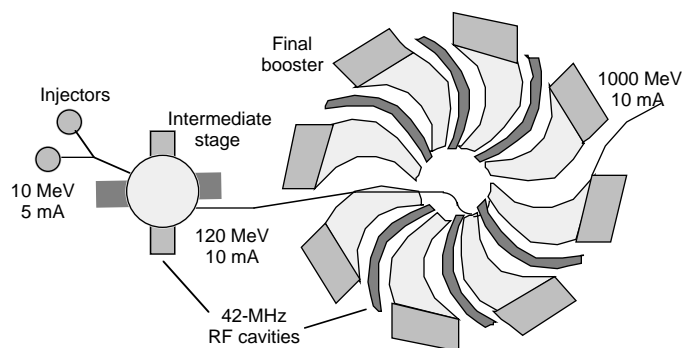
Fig. 6 CERN/PSI multi-stage cyclotron scheme for producing a 10 MW beam at 1 GeV.
