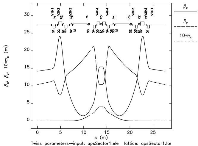
Figure 1: Advanced Photon Source Lattice
