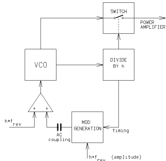
Fig. 2. Principle of the VCO drive
