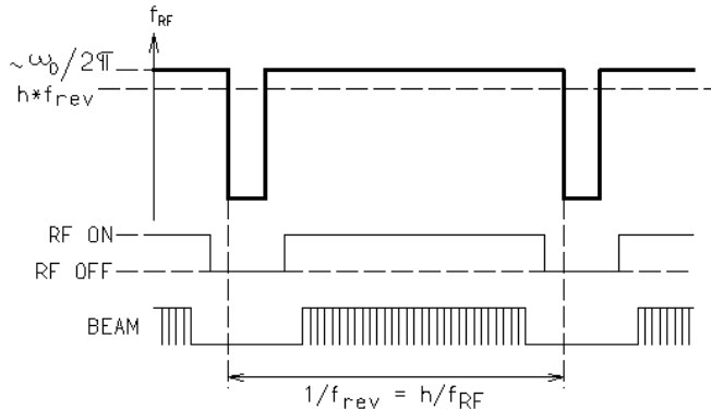
Fig. 1. FM-modulated RF
