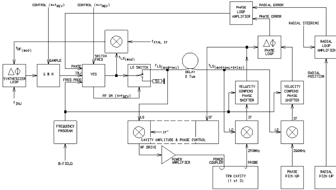
Fig. 3. Simplified block diagram of the RF system
