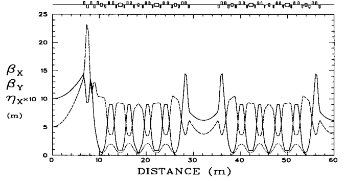
Figure. 2. Lattice OCT_5/12 (1/4 ring) with tunes \nu_x=18.37 , \nu_y=6.4 , emittance 3.6 nm.
