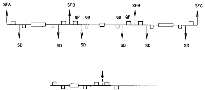
Figure 1. Lattice elements: (above) 3 C cells with a central superconducting dipole; (below) H section composed of dispersion suppressor and half straight.
