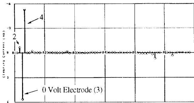
Figure 6. Display of the clearing current readback of all instrumented channels in the accumulator. The current values are differences: Channel 3 OFF - Channel 3 ON. A negative value indicates a net increase in charge cleared.
