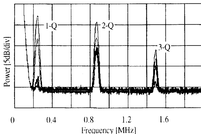
Figure 2. Vertical dipole spectrum showing coherent oscillation at the 1-q, 2-q, and 3-q betatron resonances. As the clearing voltage in accumulator sector 2 is reduced in the sequence - 900 V, 200 V, 100 V, 50 V, and 10 V, the power in each of these lines is seen to grow.
